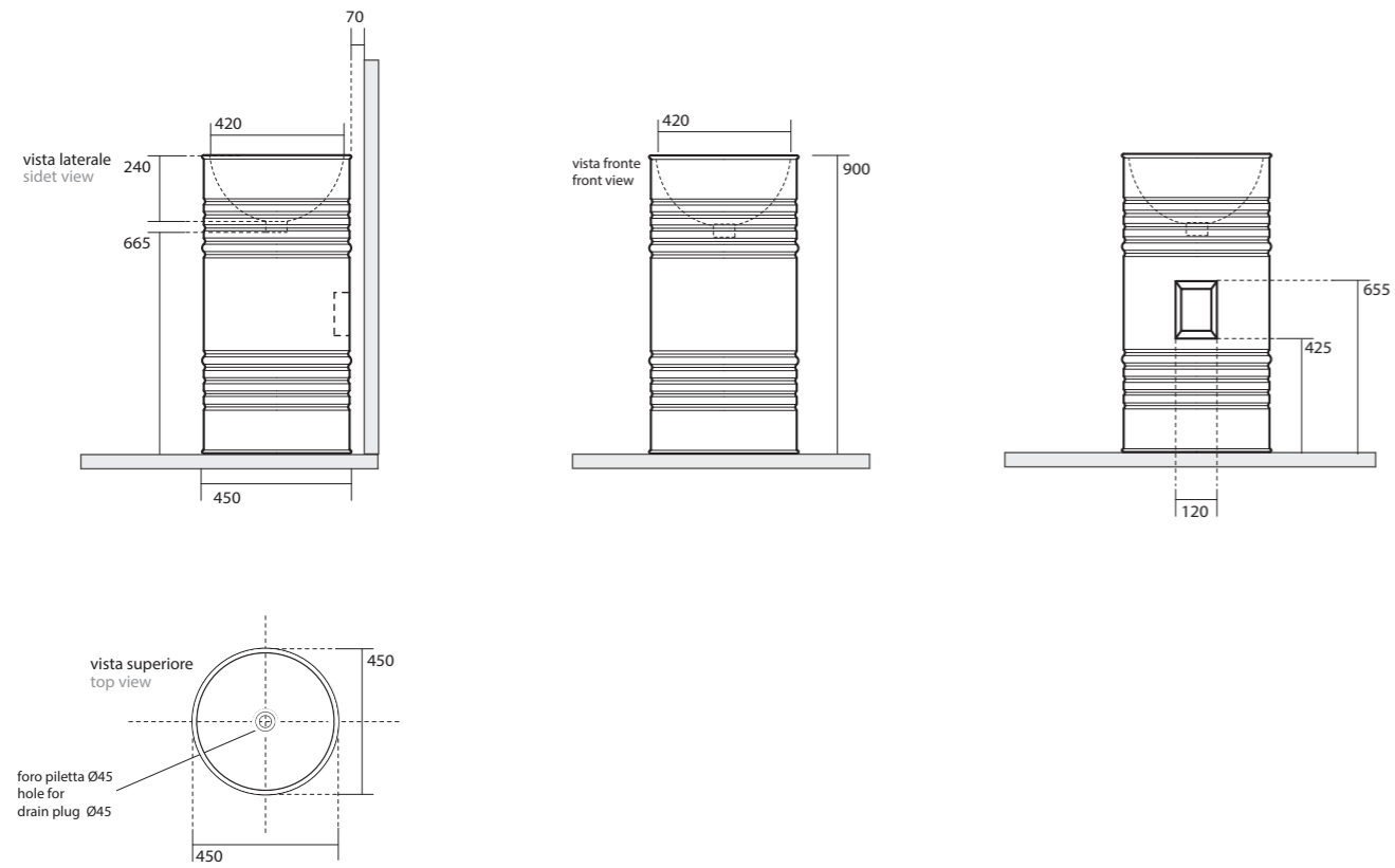
4743 Lavabo freestanding Barrel scarico a parete Freestanding washbasin Barrel wall outlet
