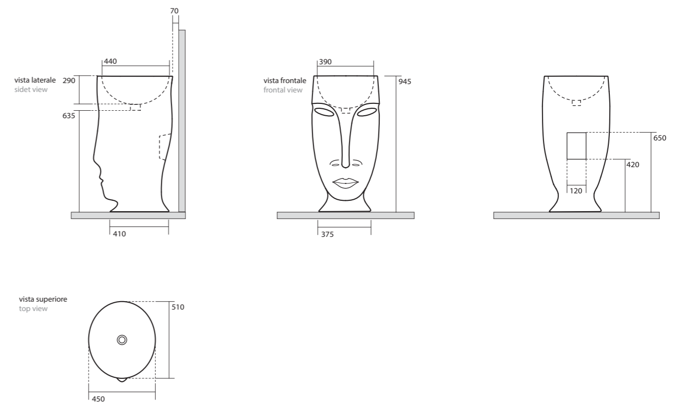
4740 Lavabo freestanding Moloco scarico a parete Freestanding washbasin Moloco wall outlet
